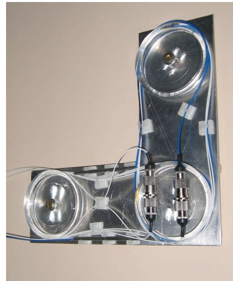
Fig. 2: Photograph of a detector showing the optical fibers forming the two orthogonal arms. See Fig. 1 for the schematic layout. The 2×2 beam splitter and joiner (Thorlabs FC632-50B-FC) are the two small stainless steel cylindrical tubes. The two FC to FC mating sleeves (Thorlabs ADAFC1) are physically adjacent. The overall dimensions of the metal base plate are 160×160 mm. The 2×2 splitter and joiner each have two input and two output fibers, with one not used. Arm 2 is folded over the splitter and joiner, compared to the schematic layout. The interferometer shown costs approximately $400.
